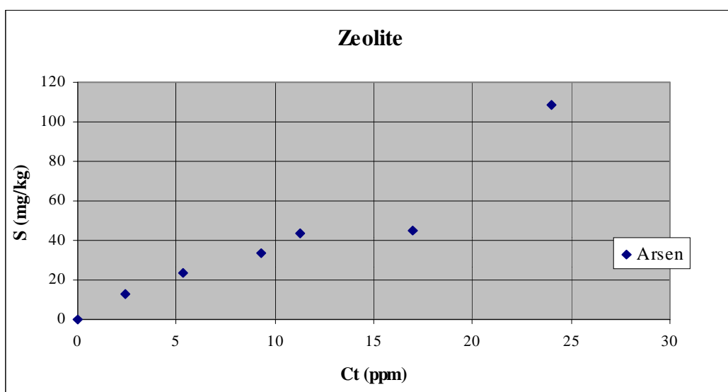
Fig. 10. Sorption of arsenic on zeolite (T: 10 °C).
