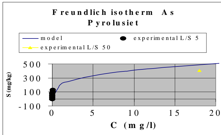
Fig. 5.1. Arsenic sorption.
