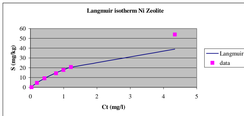
Fig. 6.3. Nickel sorption.
