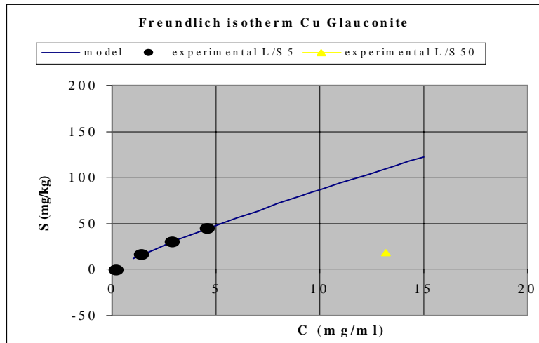
Fig. 4.2. Copper sorption.
