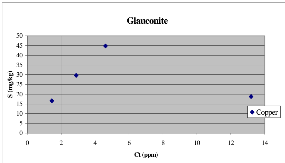
Fig. 3. Sorption of copper on glauconite (T: 10 °C).
