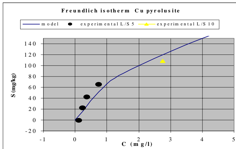
Fig. 5.2. Copper sorption.
