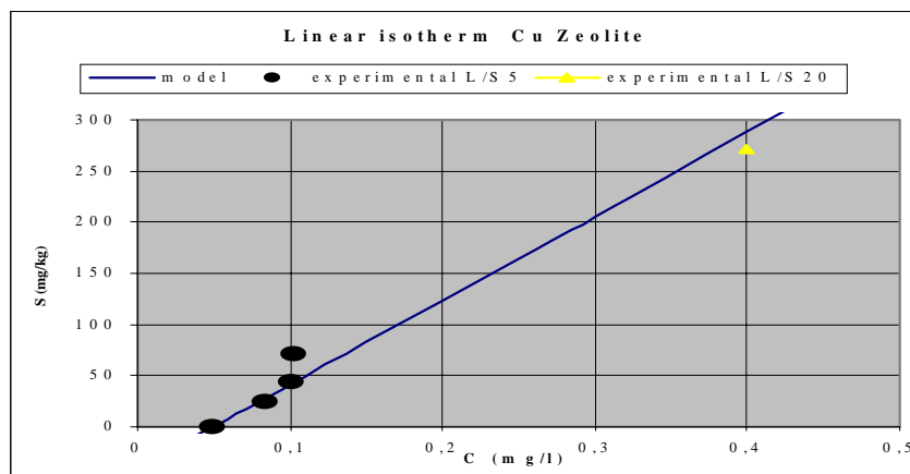
Fig. 6.2. Copper sorption.
