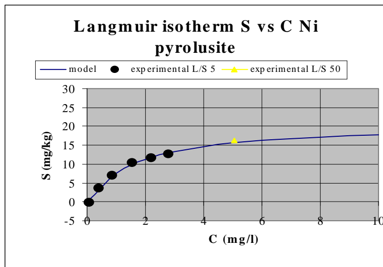
Fig. 5.3. Nickel sorption.
