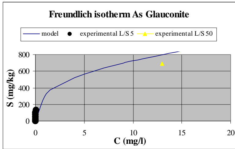
Fig. 4.1. Arsenic sorption.
