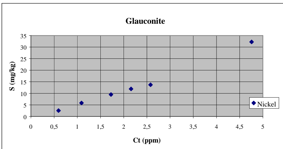
Fig. 4. Sorption of nickel on glauconite (T: 10 °C).
