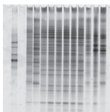
Figure 2. Denaturing Gradient Gel Electrophoresis (DGGE) of bacterial communities in a river basin profile
